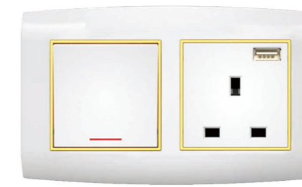
13A 250V~ 3 PIN SOCKET WITH USB+45A WATER HEATER SWITCH 7x14
